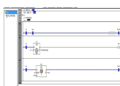
Figure 3 Ladder diagram-level 3
