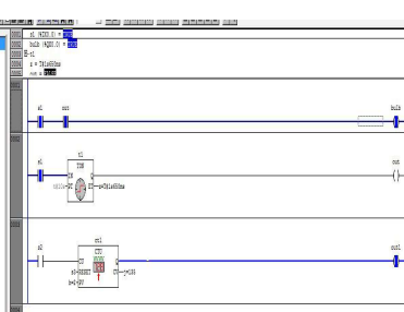
Figure 2 Ladder diagram-level 2
