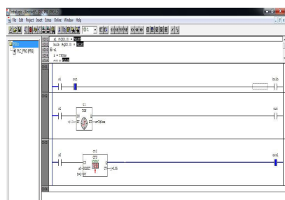
Figure 1 Ladder diagram-level 1
