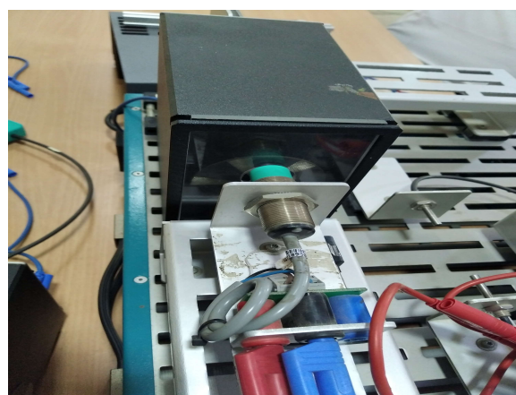
Figure 7: Magnetic sensor (Proximity sensor) aligned in front of the rotary target coupled with motor.
