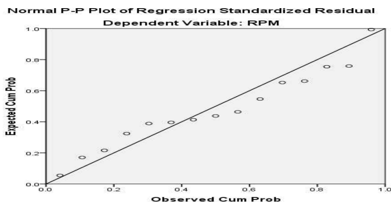
Figure 9: Normal P-P plot of Regression standardized residual
