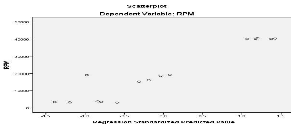
Figure 10: Scatter plot of Regression
