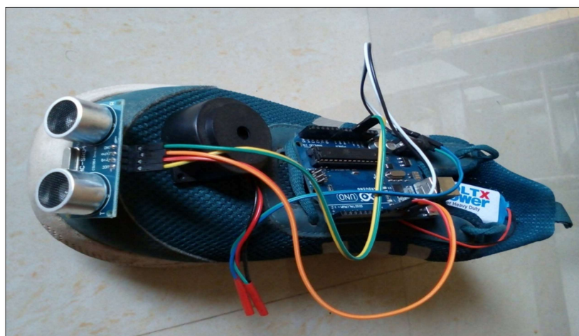
Figure 7: Hardware Implementation
