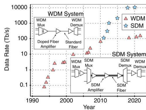
Figure3: Evolution of data rate records for WDM systems since 1996 and SDM systems
