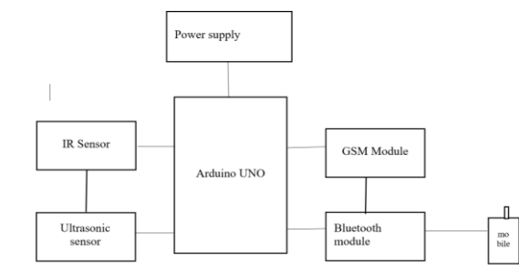
Figure 1: Proposed Methodology
