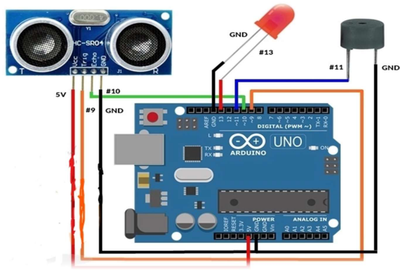
Figure 6: Circuit diagram
