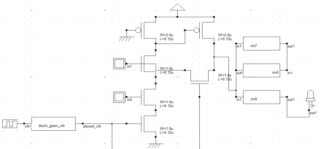
Figure 2(a) Schematic of the proposed P-FF des
