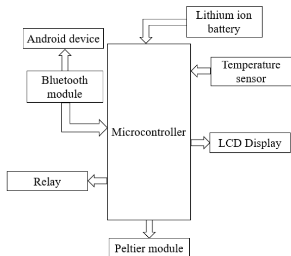
FIGURE 1. SCHEMATIC DIAGRAM OF THE INTEGRATED COOLWARM JACKET
